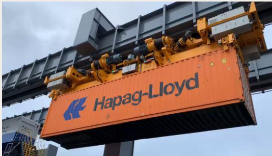
En-route Sky Rail Inspection Solution
