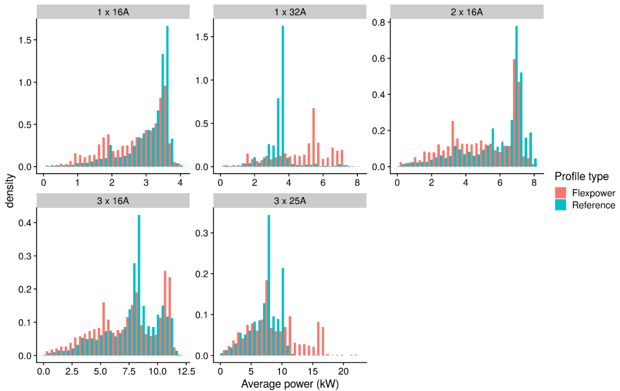
Figure 4: Distribution of the average power per transaction per vehicle category for Flexpower and reference stations. The average is calculated for the whole session, so periods of slower charging during the current limitation can be compensated in the preceding or following hours. Only sessions that have not finished charging upon disconnection are shown (47.3%).
