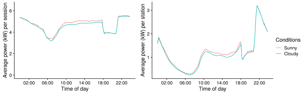
Figure 5: The average power per active session and per station over the day for different weather conditions.
