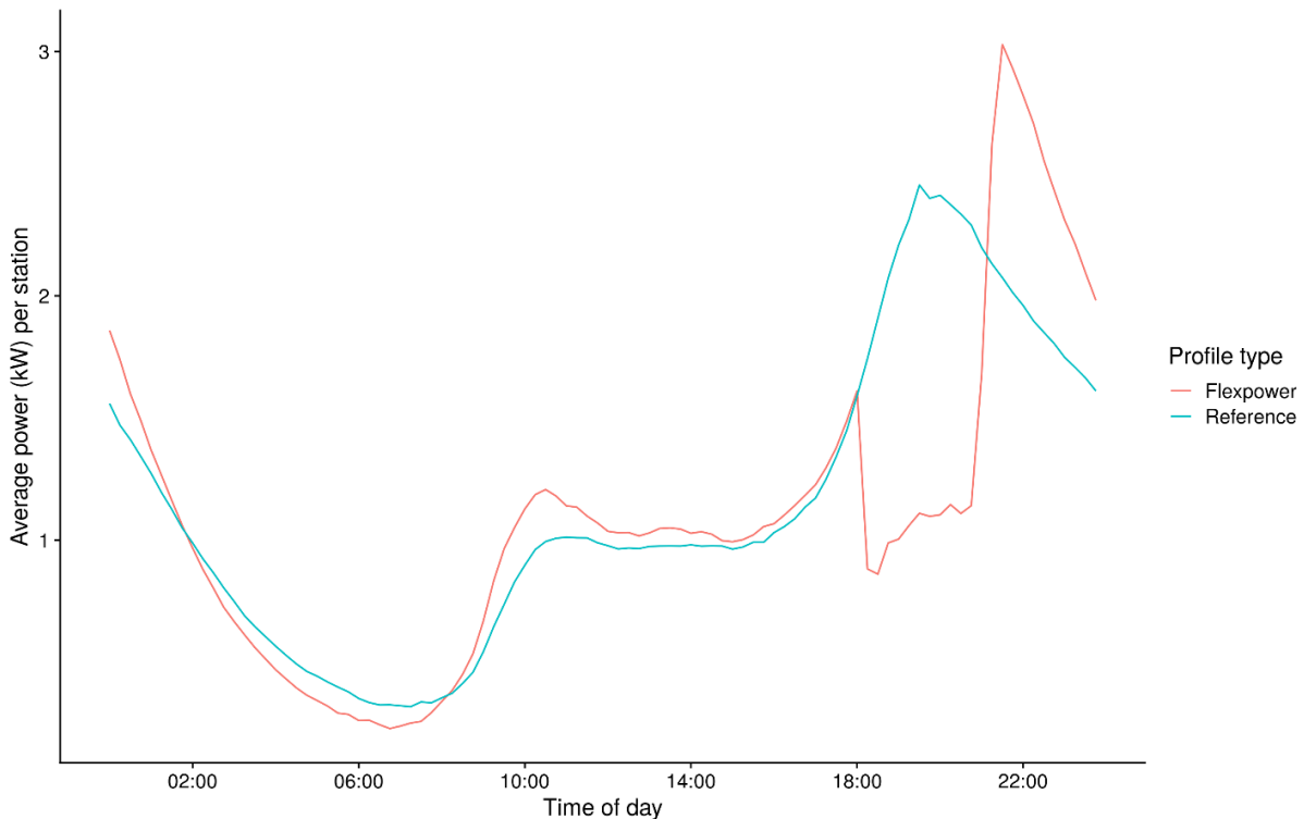
Figure 3: The average power per station over the day for Flexpower and reference stations. The plotted value represents the total grid load contribution of EV charging.
