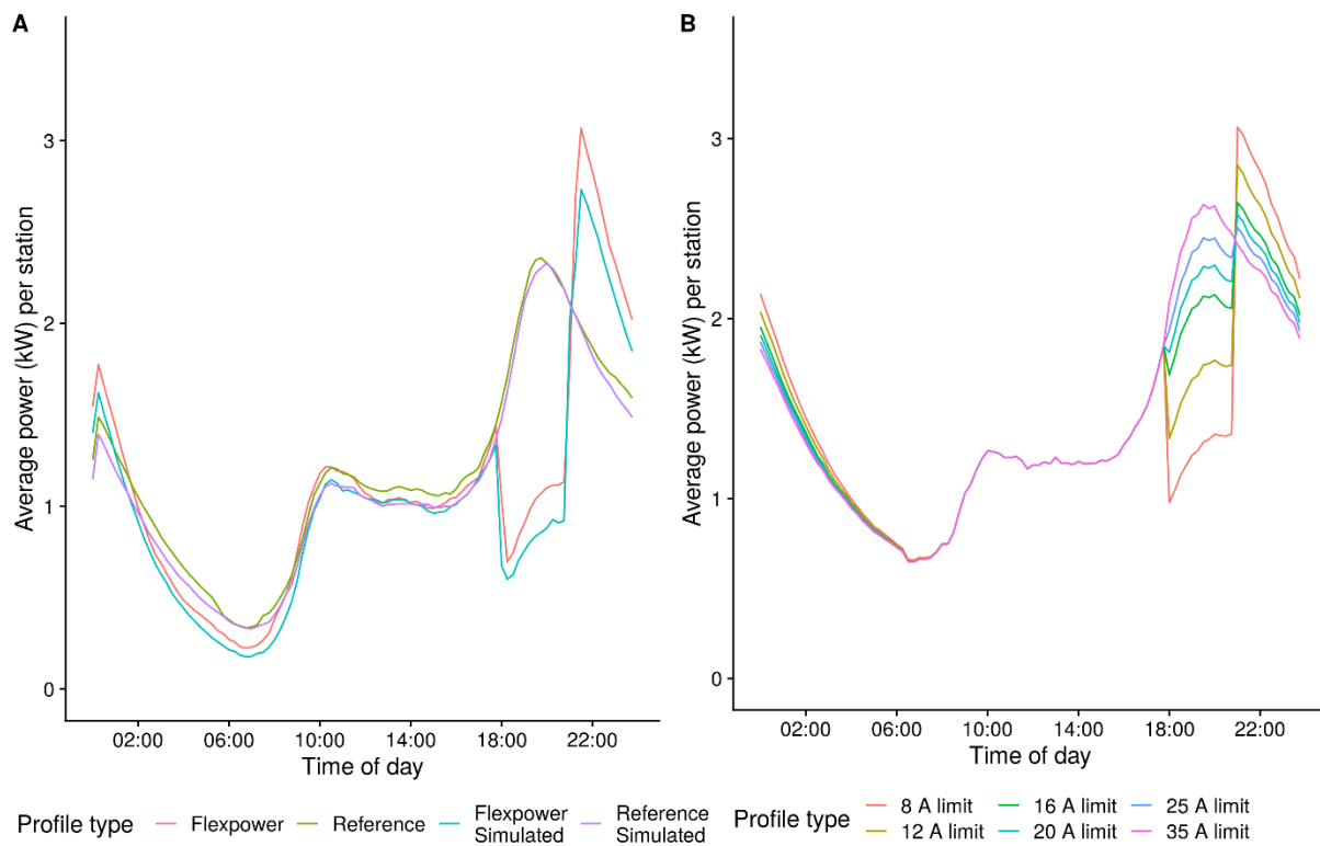
Figure 6 A: Average charging power per station for the actual data on Flexpower and reference stations, as well as a simulation of the Flexpower and reference profiles on the same transactions. B: Simulations of the average charging power per station on a fixed set of transactions using different current limitation levels during the evening hours (18:00 – 21:00).
