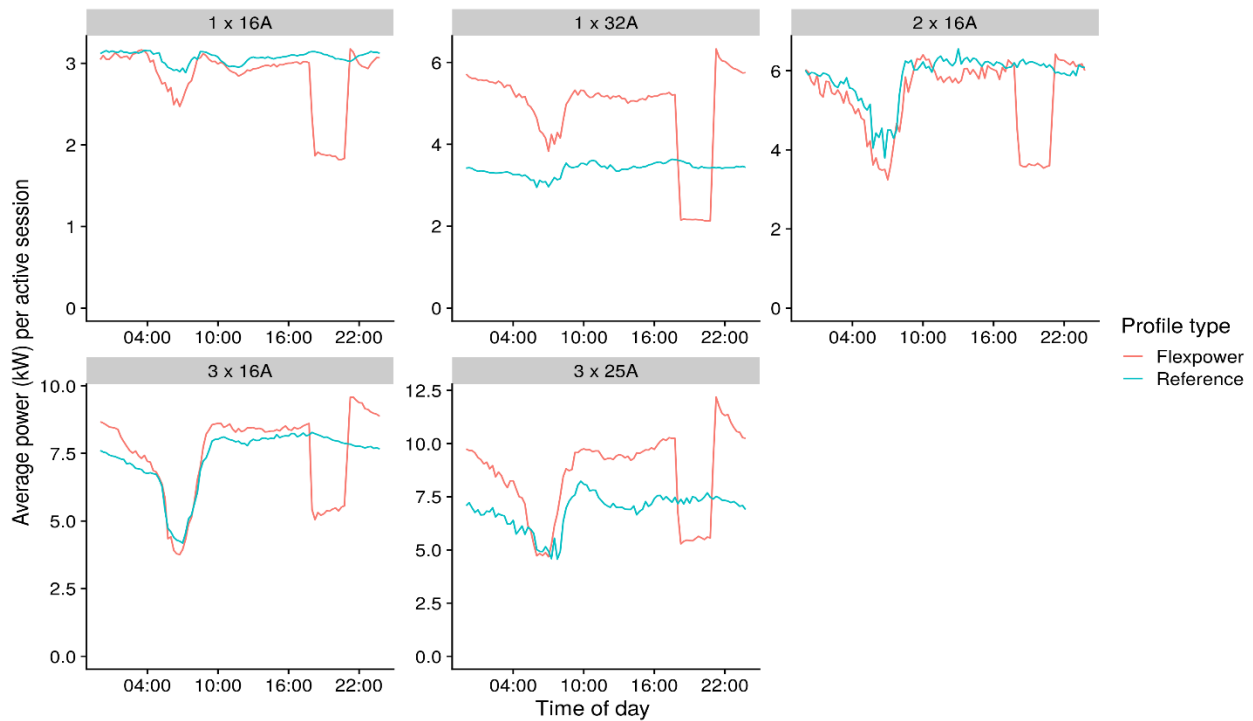
Figure 2: The average power over the day for the different vehicle categories during charging. The resolution of the graph is 15 minutes, which is limited by the resolution of the data.
