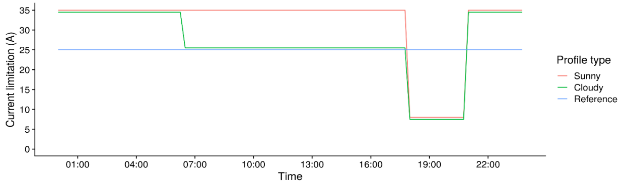
Figure 1: The time-dependent profile deployed on the selected Flexpower charging stations under sunny and cloudy conditions compared to the current limit per phase on a regular public charging station in Amsterdam.
